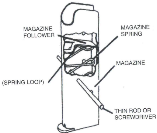
FIGURE-11 MAGAZINE ASSEMBLY WITHOUT REMOVABLE BASE
