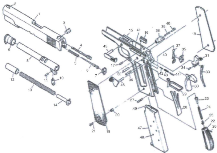
FIGURE 12-BLK 1911 PARTS ILLUSTRATION
