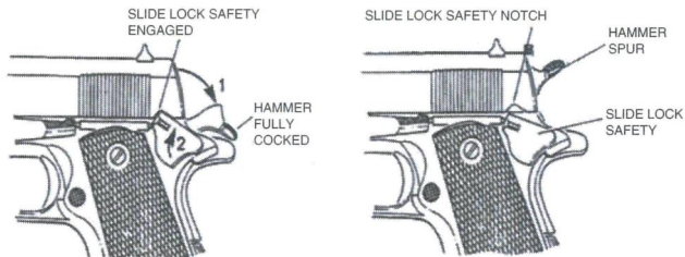
FIGURE 2- SLIDE LOCK SAFETY
