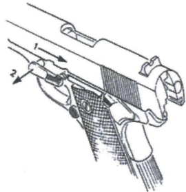
FIGURE 7 REMOVING SLIDE STOP
