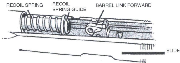
FIGURE 8 - BARRELLINK MUST BE FORWARD ONLY FOR BARREL TO BE REMOVED AND ASSEMBLED THROUGH THE SLIDE
