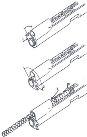
FIGURE 9 - INSTALLING BARREL BUSHING AND RECOIL SPRING/S
