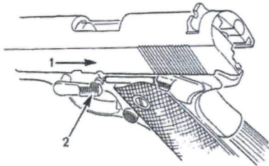
FIGURE 10 -INSTALLING SLIDE STOP
